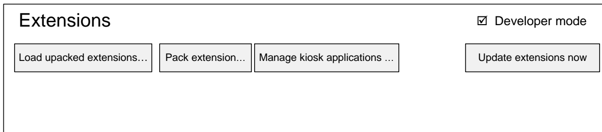
Figure 14. Extensions Screen
